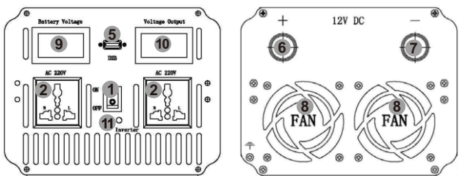
BEP800S/BEP1500S/BEP2000S/BEP3000S面板示意图
