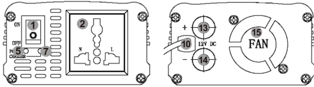
BEU500L/600L/800L/1000L UPS Panel Diagram
