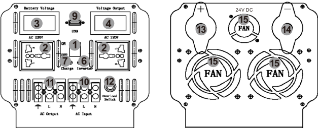
BEU5000L UPS Panel Diagram
