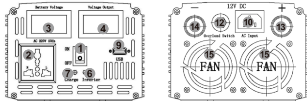
BEU2000L/3000L UPS Panel Diagram
