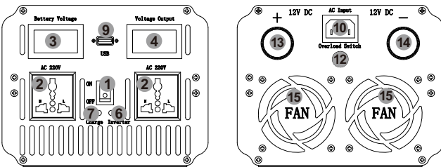
BEU5000L UPS Panel Diagram
